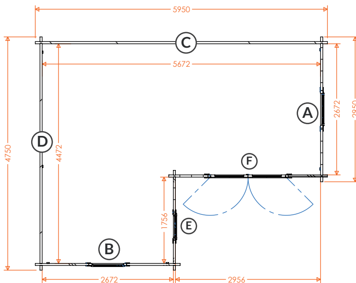
20x16w Lana 44mm 2016LAN-44
