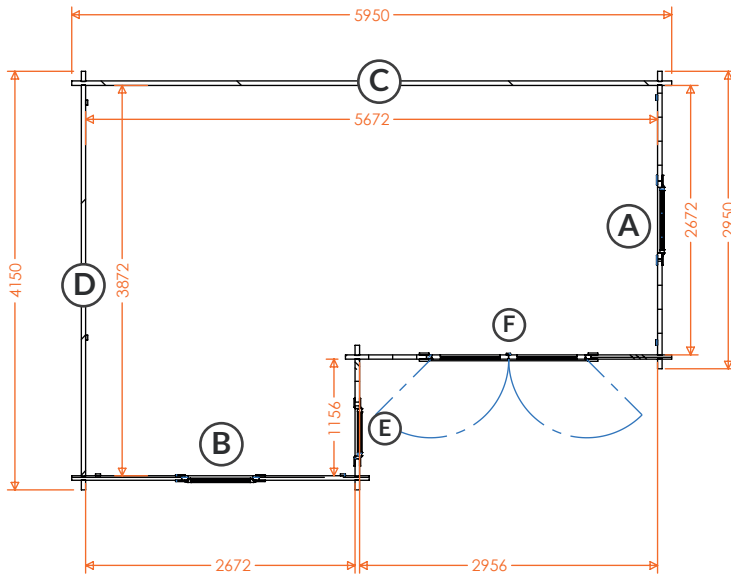
20x14w Lana 44mm 2014LAN-44
