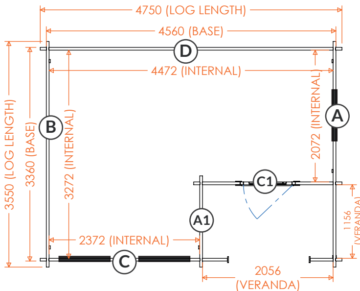
16x12w Amur 44mm 1612SIG-44
